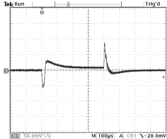
Figure 20. Vin=5V, Vout=1V. Bandwidth is 40kHz
