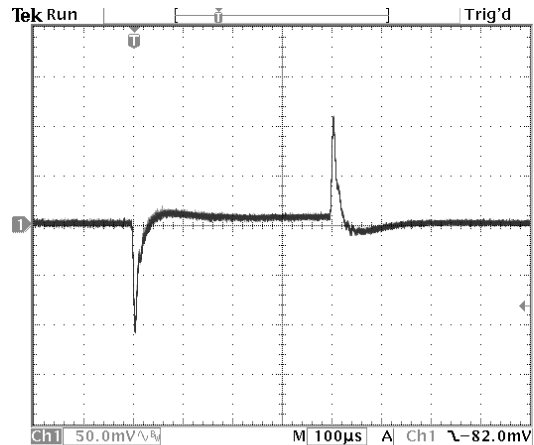
Figure 21. Vin=5V, Vout=2.5V. Bandwidth is 40kHz
