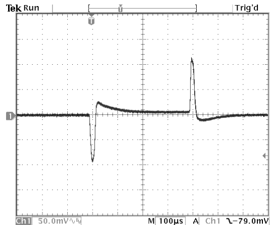
Figure 22. Vin=3V, Vout=1V. Bandwidth is 30kHz
